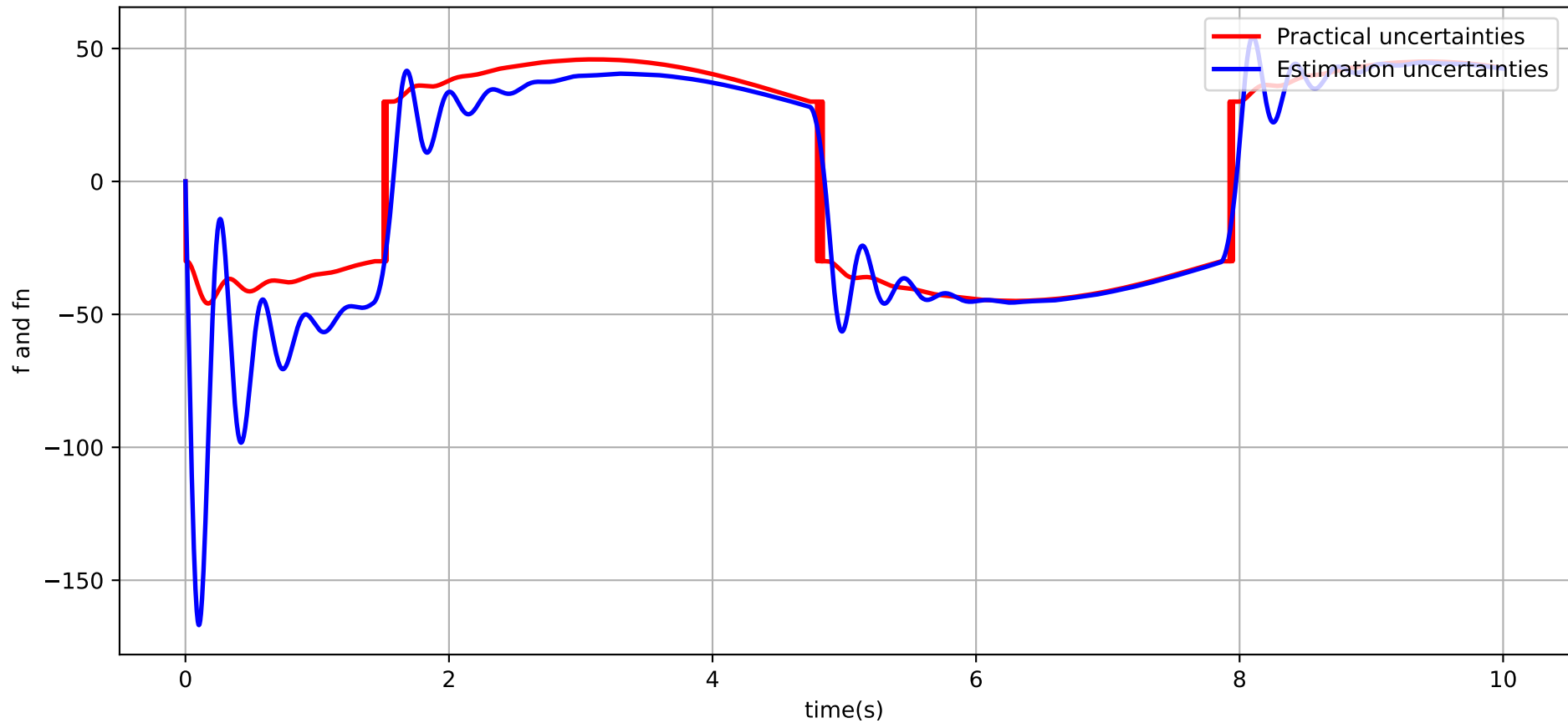
Disturbance Estimation Performance ( S=3 , S1=2 , m=50 )
